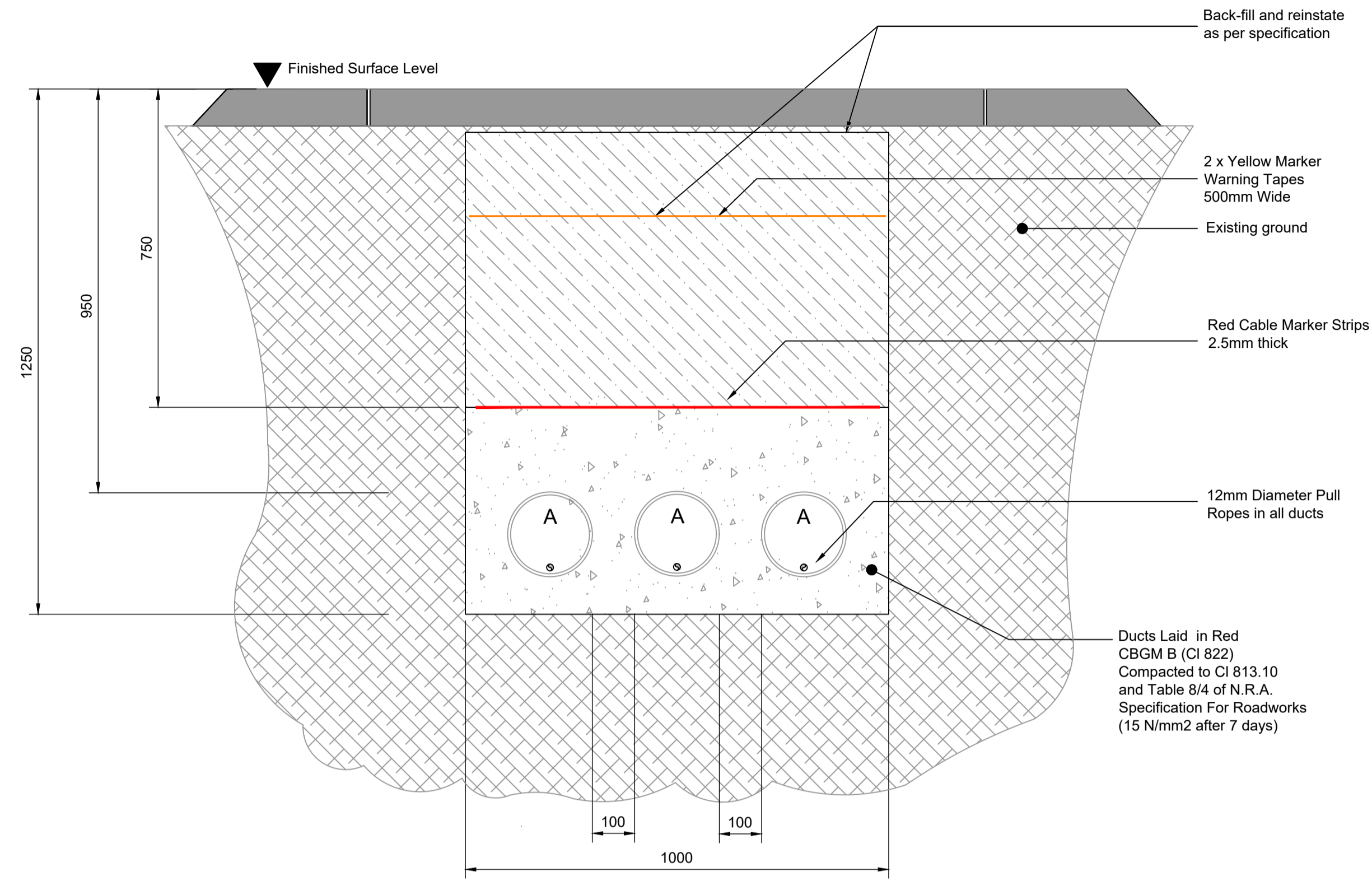
220kV Cable Trench - Typical Arrangement
